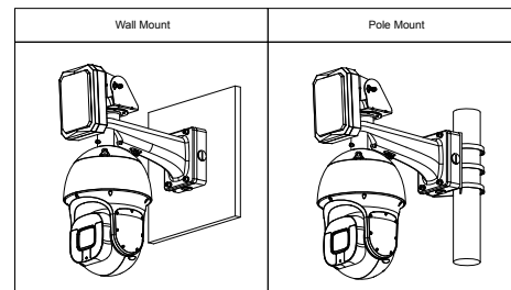
PFA150 Pole Mount Bracket
