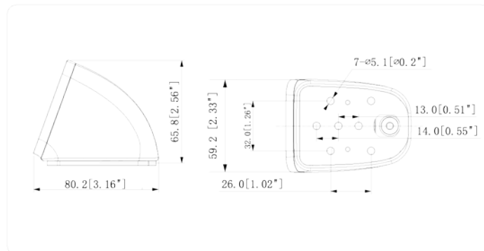
Device dimension (mm [inch])
