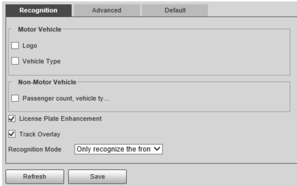
Figure 5-28 Recognition
