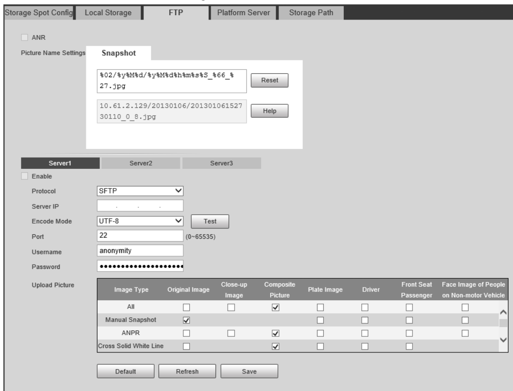
Figure 5-48 FTP
