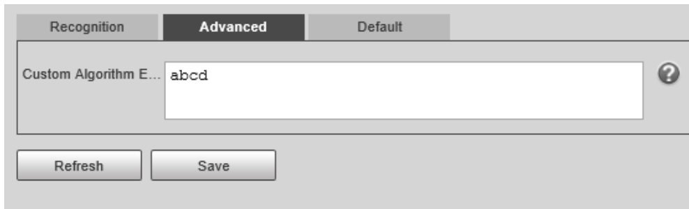
Figure 5-29 Custom algorithm
