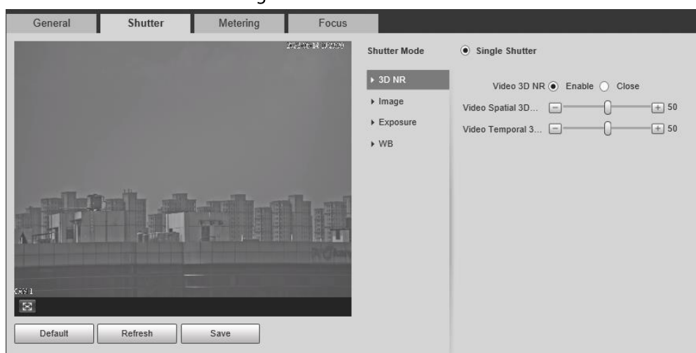
Figure 5-2 Shutter
