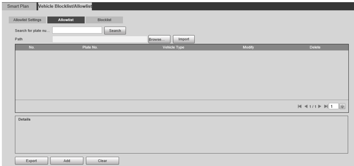
Figure 5-16 Allowlist
