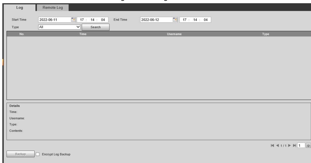
Figure 5-67 Log
