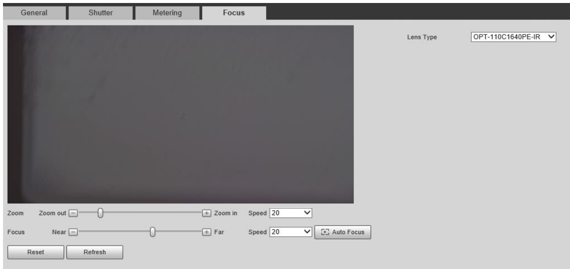
Figure 5-4 Focus
