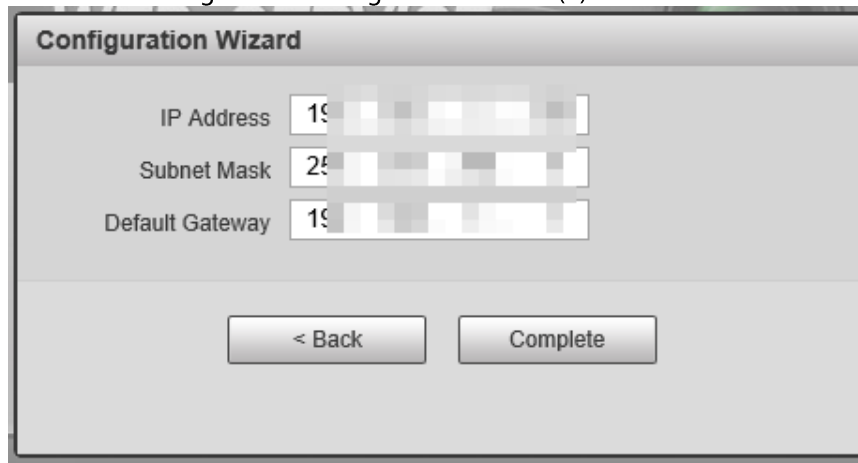
Figure 1-7 Configuration wizard (2)
