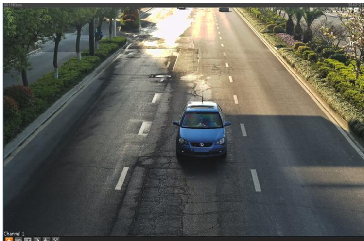
Figure 2-2 Big window
