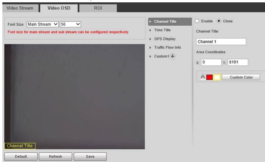
Figure 5-6 Video OSD
