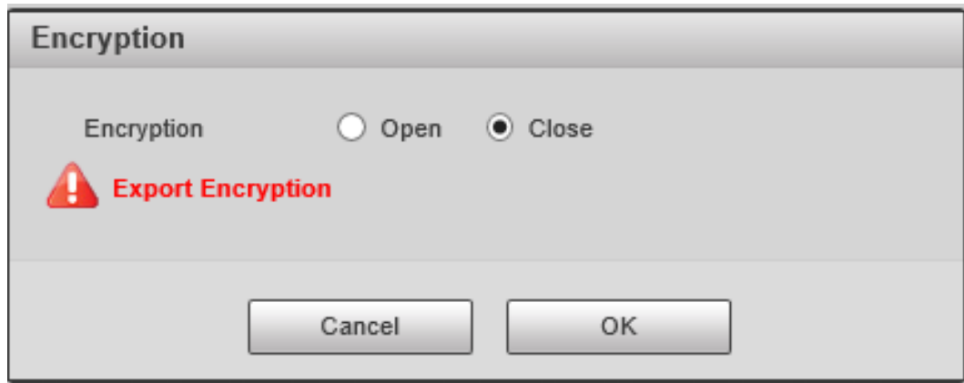
Figure 5-18 Encrypt configuration
