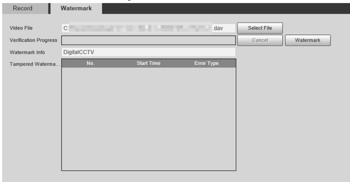
Figure 4-6 Watermark
