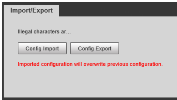
Figure 5-64 Import/Export
