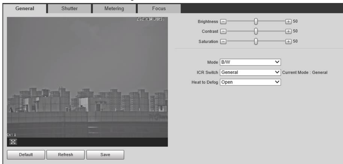
Figure 5-1 General
