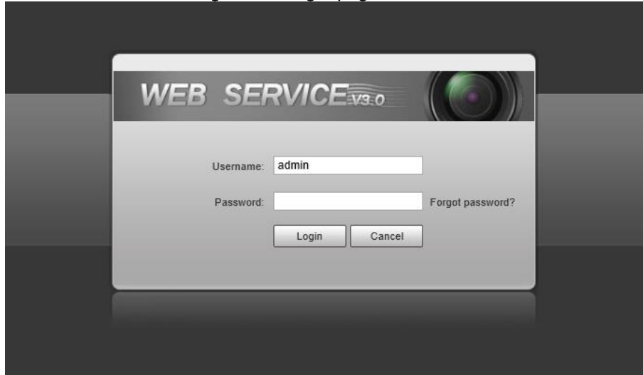
Figure 1-5 Login page
