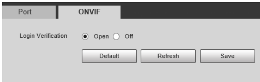
Figure 5-10 ONVIF
