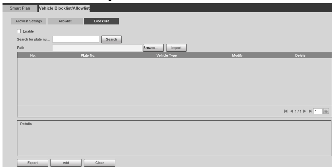
Figure 5-19 Blocklist search
