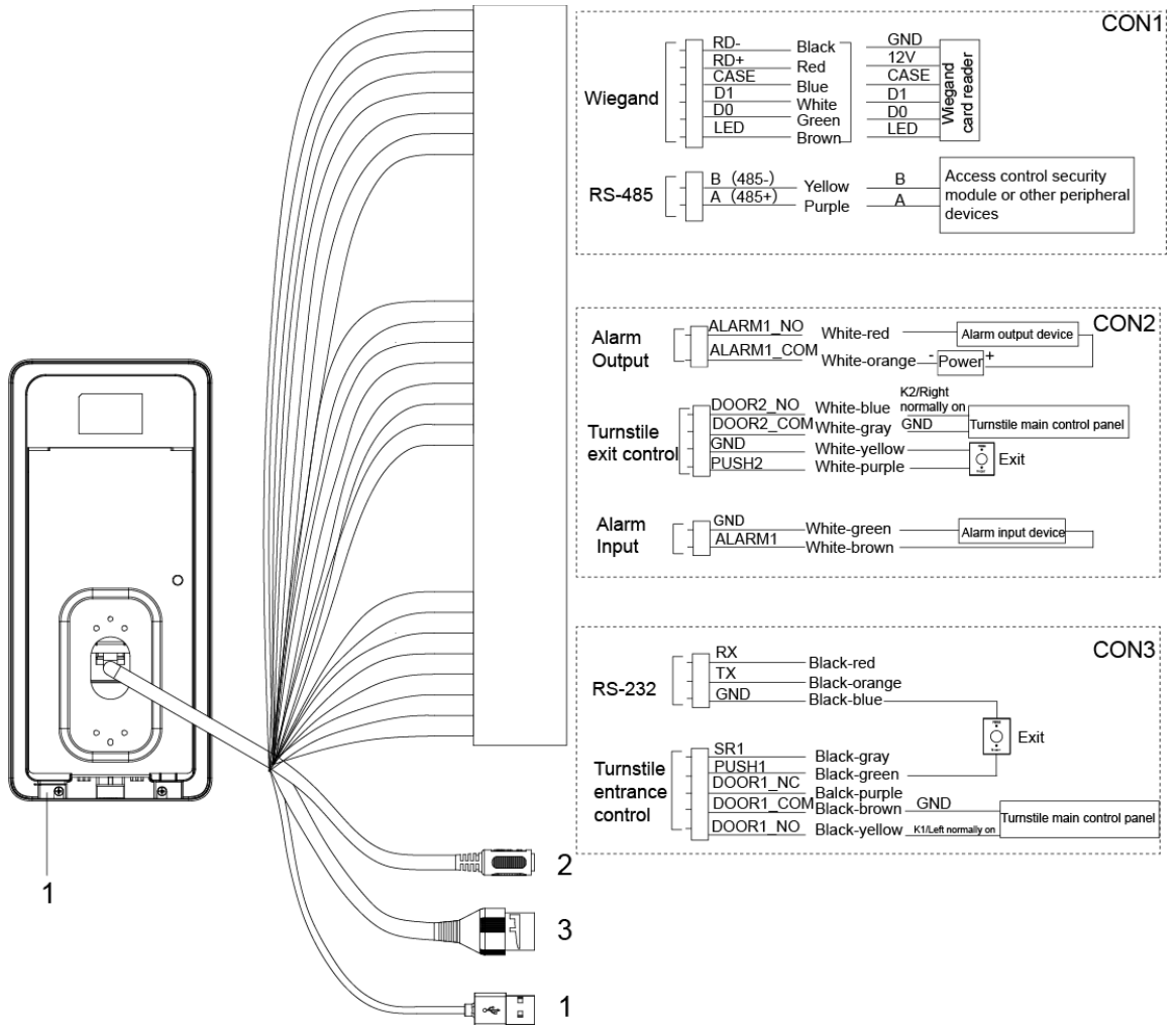
Figure 2-5 Cable connection
