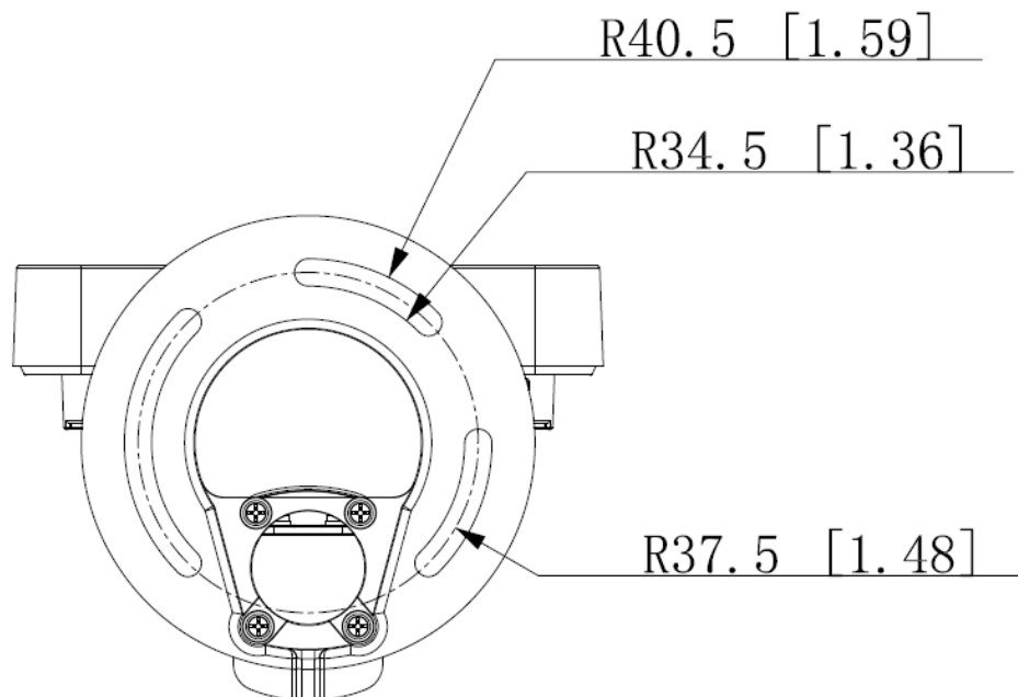
Figure 2-4 Installation drawings (mm[inch])
