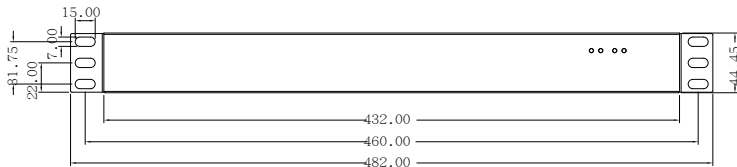
Mounting Bracket
