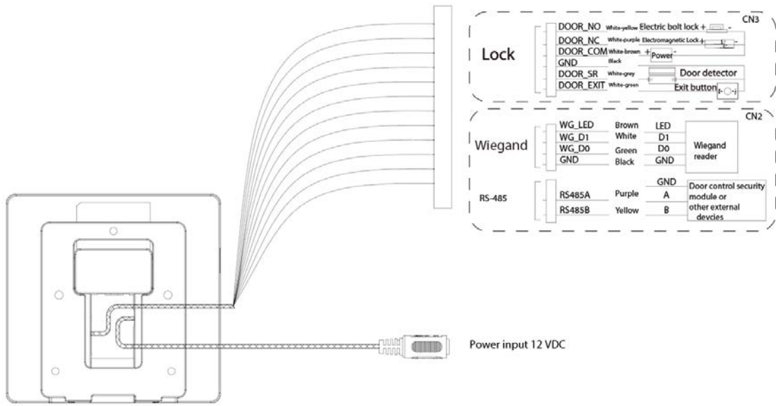
Figure 2-5 Wiring
