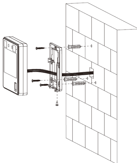
Figure 2-6 Wall mount
