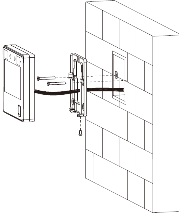
Figure 2-7 86 box mount
