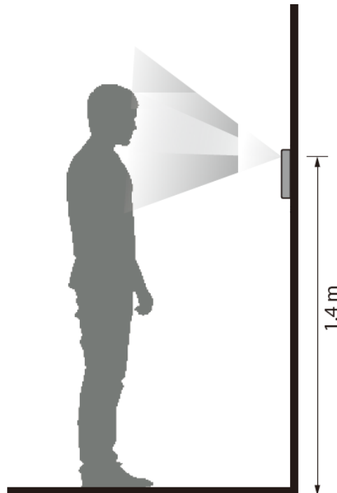
Figure 2-1 Installation height requirement
